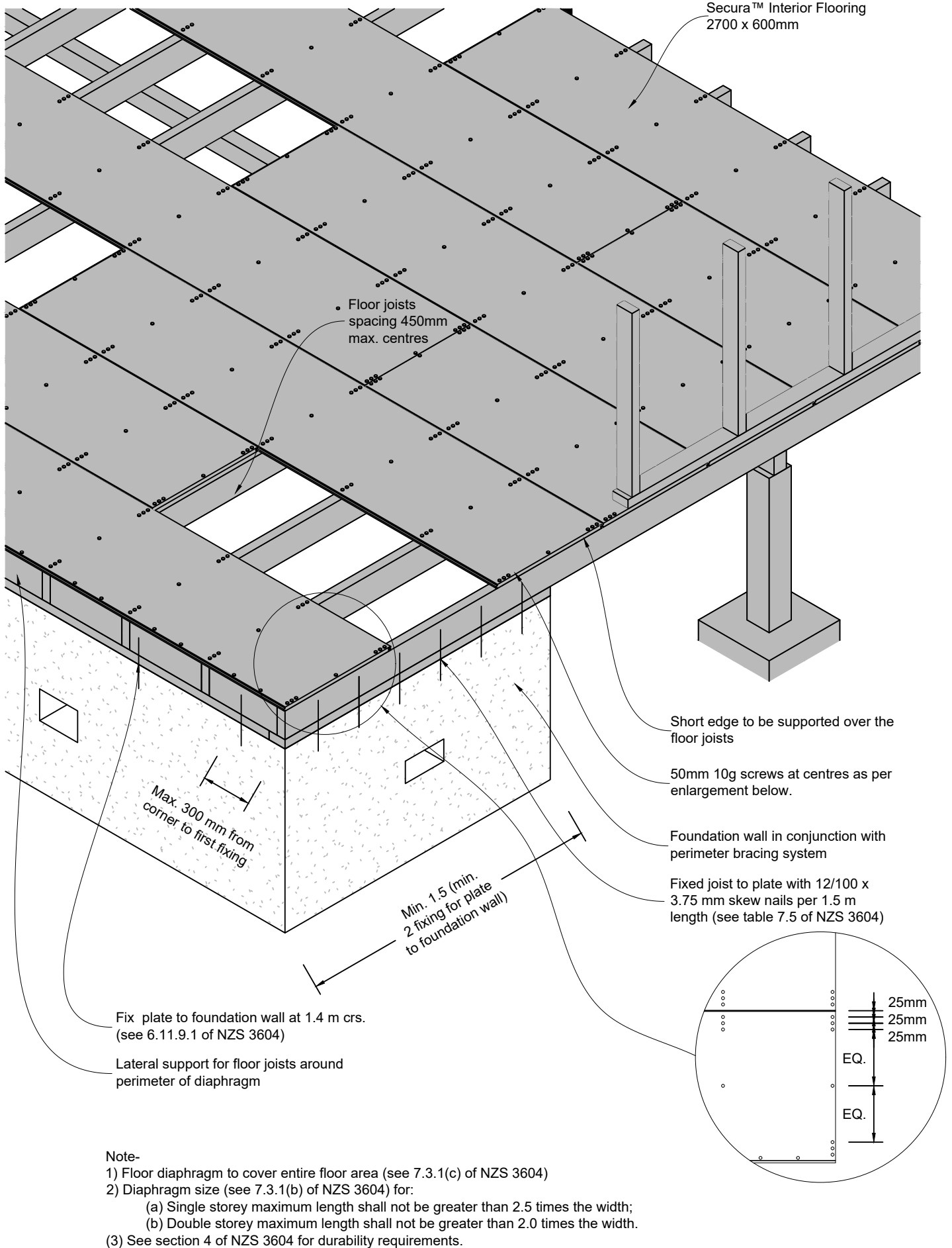
fig19 jhl_brce_wall_secu.dwg
